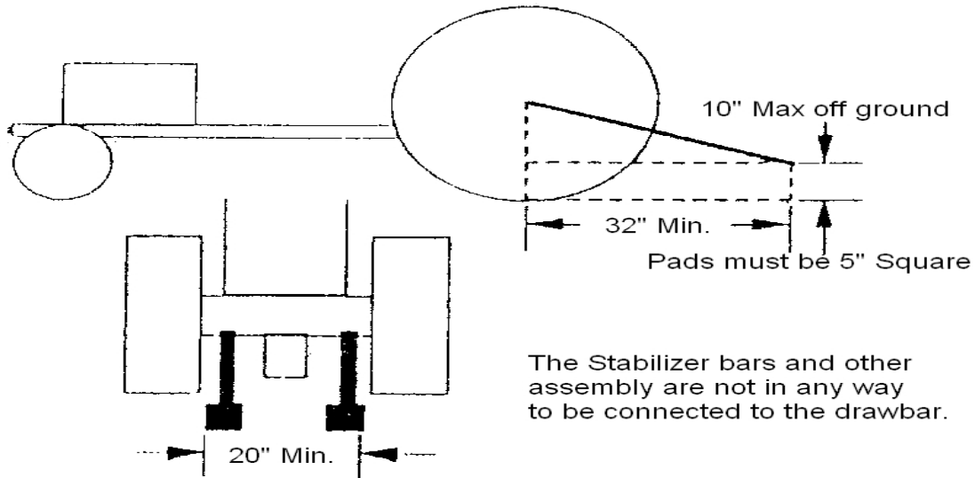
Example: Stabilizer Bar
